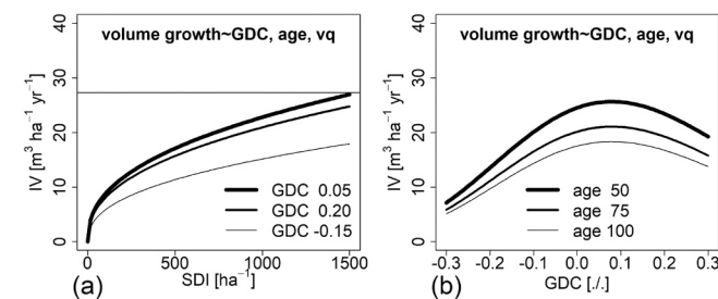
Fig. 10. Stand volume growth, IV , increases with stand density, SDI , and is additionally modulated by the growth partitioning, GDC . Visualization according to model 5 (see model coefficients in Table 7). (a) IV - SDI relationship shown for GDC = 0.05, 0.20, -0.15 ( vq set to 1.0, stand age to the mean of 50 years). (b) unimodal IV - GDC relationship shown for age 50, 75, and 100.
